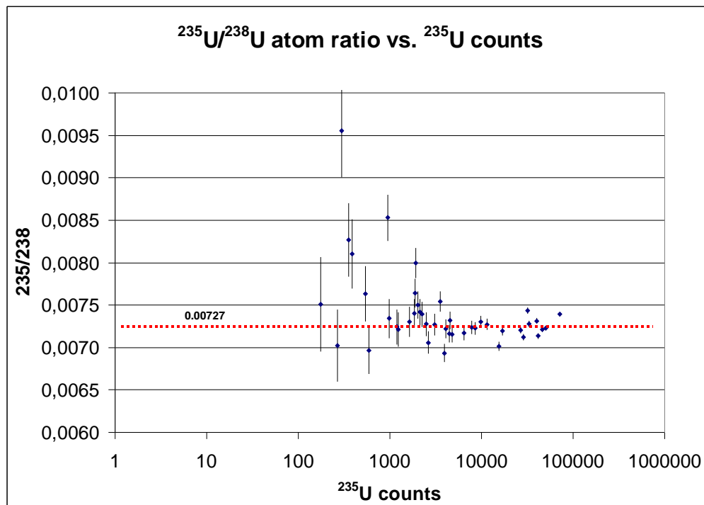
Figure 16. The dependence of the analyte concentration in determination of the ^{235}\text{U}/^{238}\text{U} ratio. The sensitivity of the instrument was such that 1000 ^{235}\text{U} counts corresponded to a concentration of 0.1 ppt natural uranium.
