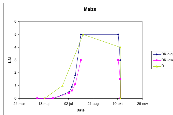
Fig. 4.7. LAI for maize. Estimates used by default in ECOSYS (D) and in the Danish model (DK) for high and low fertilisation status.
