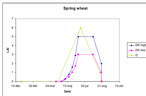
Fig. 4.3. LAI for spring wheat. Estimates used by default in ECOSYS (D) and in the Danish model (DK) for high and low fertilisation status.
