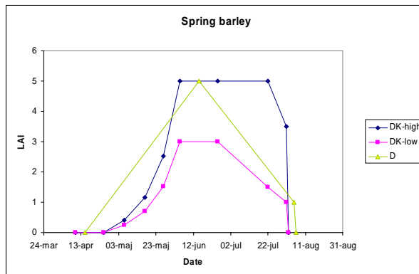
Fig. 4.5. LAI for spring barley. Estimates used by default in ECOSYS (D) and in the Danish model (DK) for high and low fertilisation status.
