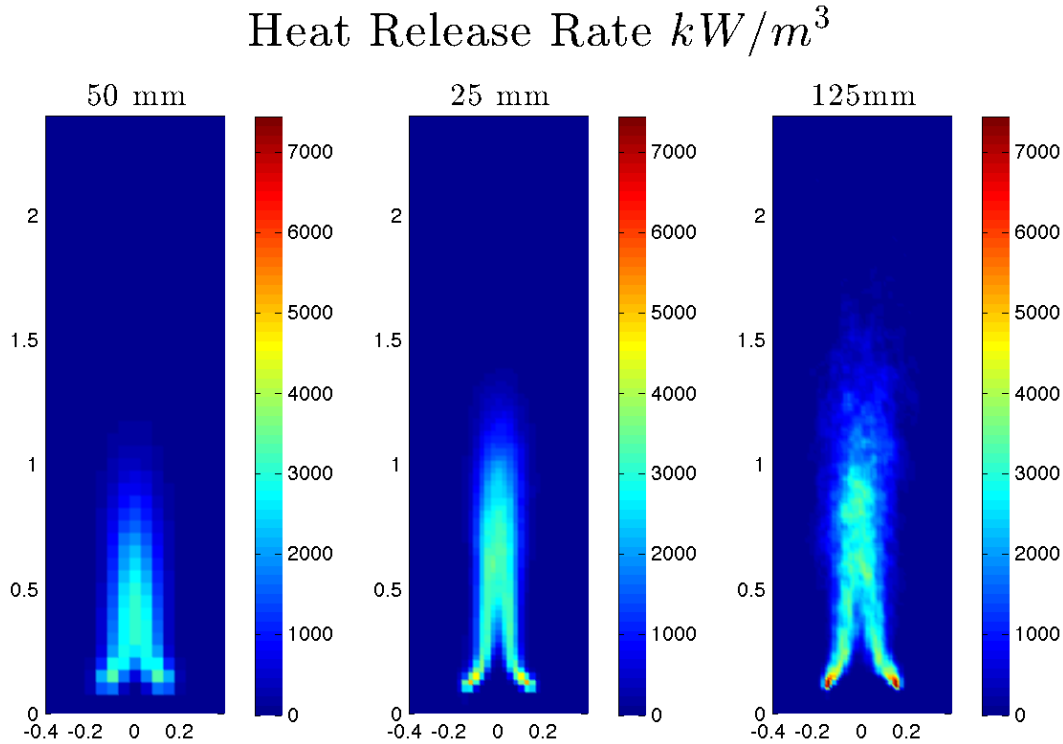
Figure 42. HRRPUV slices for three different grid resolutions
