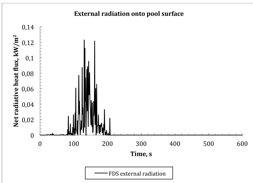
Figure 77 Net radiative heat flux onto pool surface.
