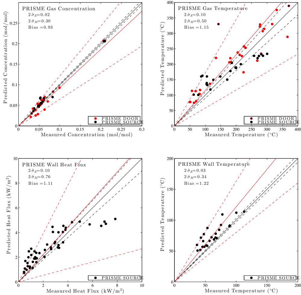
Figure 60. Measured vs. predicted quantities in the PRISME SOURCE and PRISME DOOR test series. Simulations with predicted HRR
