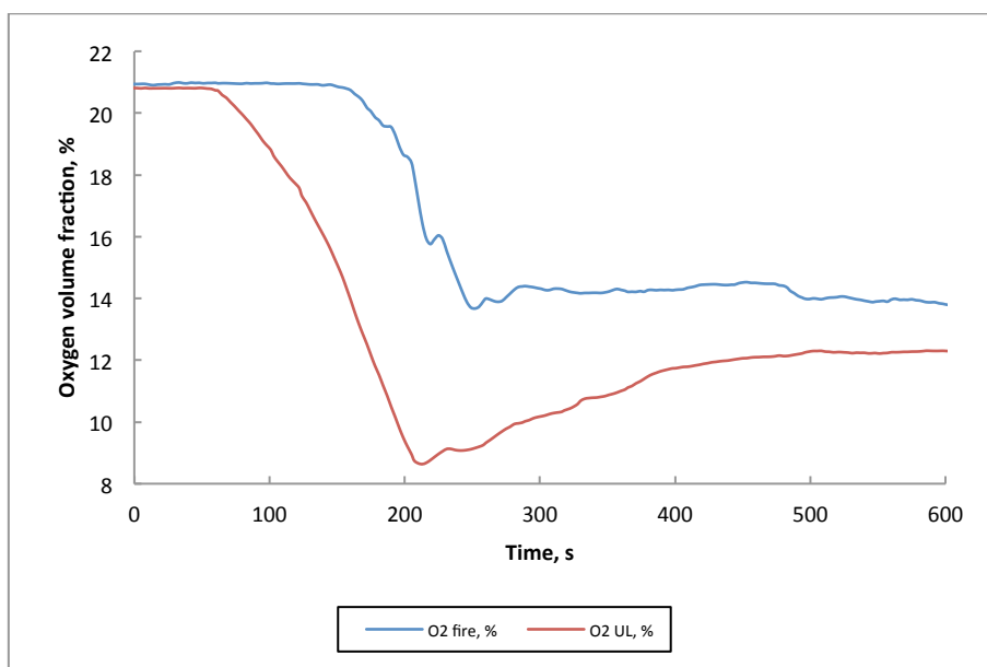
Figure 73 Oxygen concentration (dry air) close to the fire source and in the upper layer, test 6.
