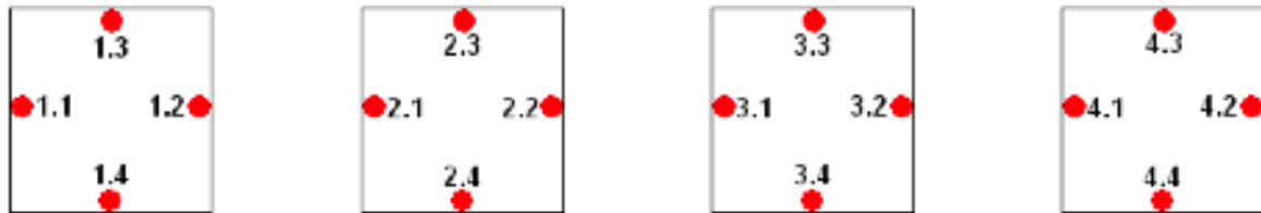
Figure 47 Numbering of thermocouples in the pipes
