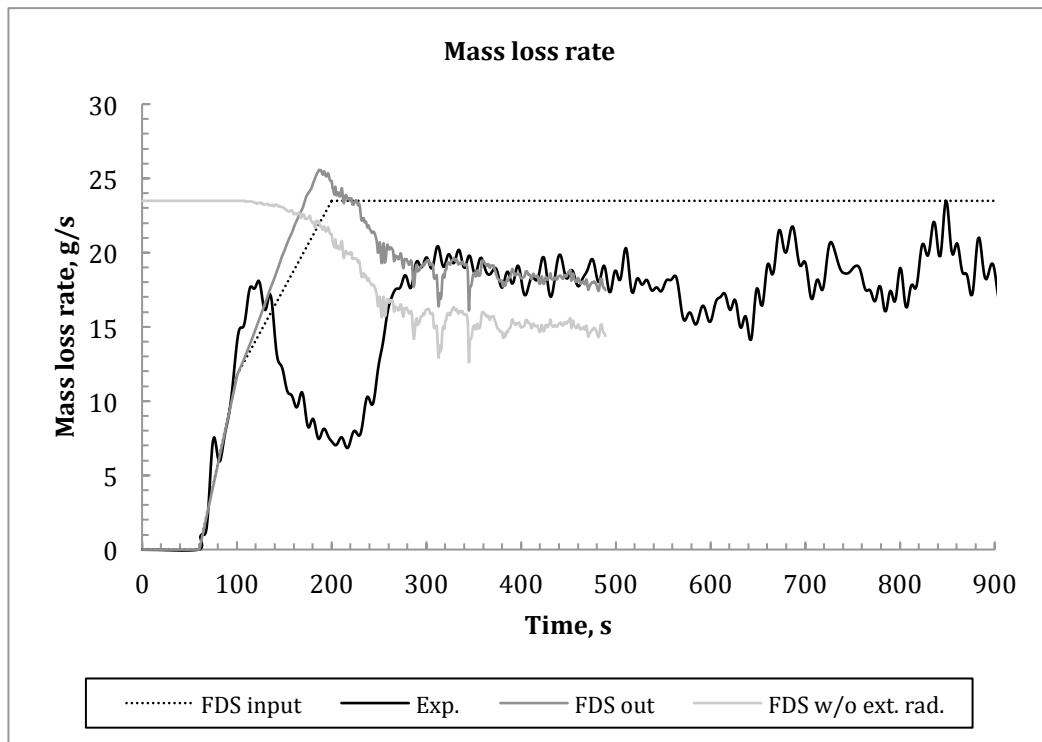
Figure 62 Prediction and test results of the mass loss rate in LEAK1 test
