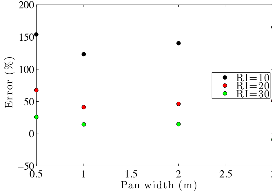
Figure 57. Error in predicted mass loss rate (MLR) as function of pan width and Resolution Index (RI)
