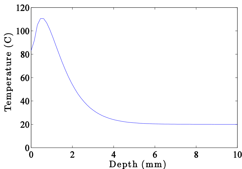
Figure 39 Instantaneous temperature profile within a pool of heptane with the radiation heat transfer within the liquid.
