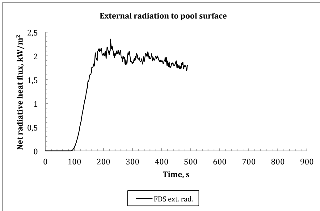
Figure 64 Simulation results of the net radiative heat flux to the pool during LEAK1 test simulation
