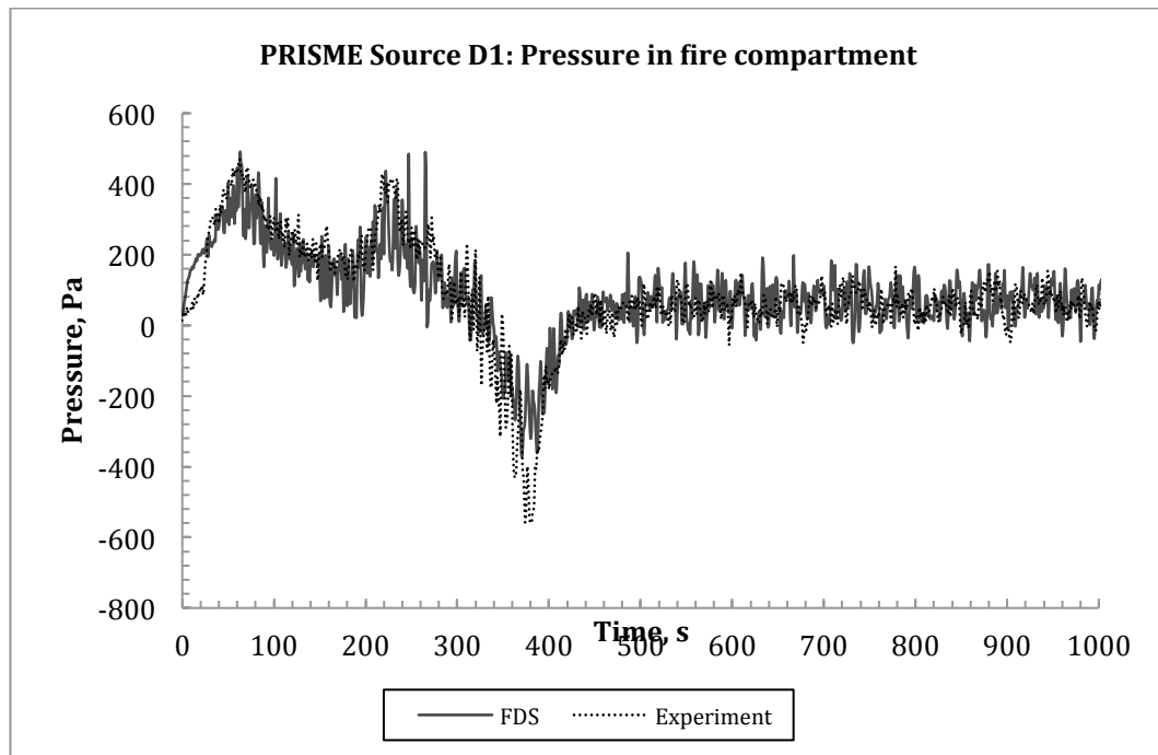
Figure 16 The predicted pressure inside the fire compartment compared to the experimental data from test Source D1 (SI_D1).
