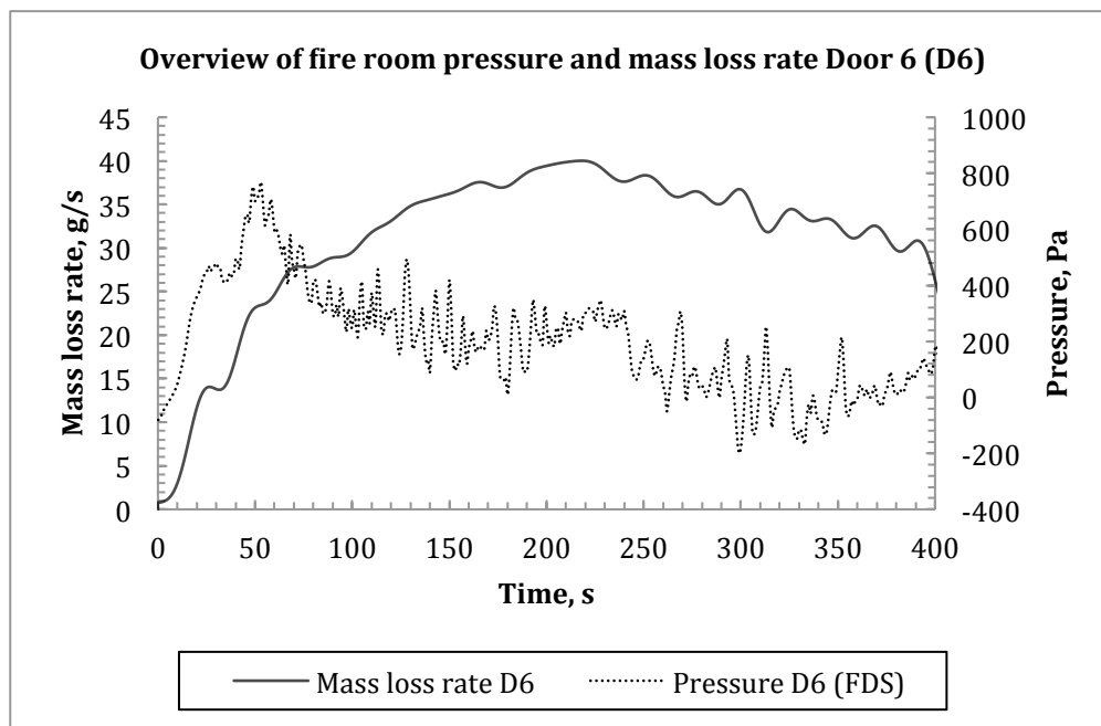
Figure 35 Overview of fire room pressure and mass loss rate during (MLR) test Door 6 (D6).
