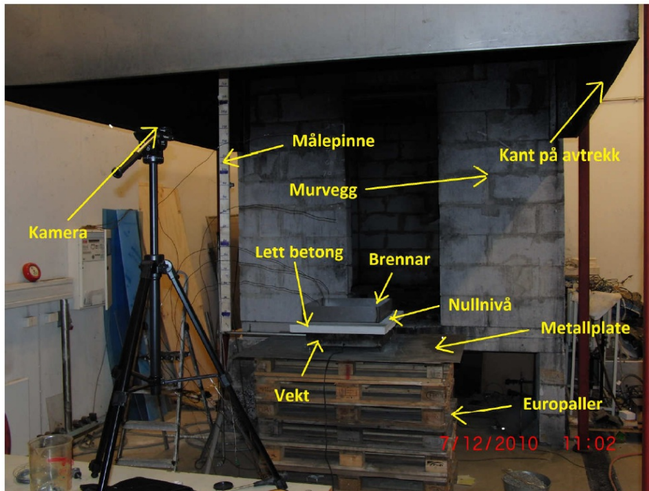
Figure 46 Set-up in Haugesund for pool fire experiments
