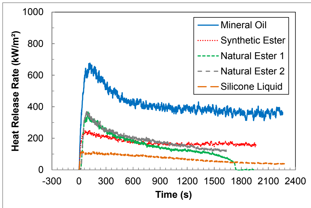
Figure 51 HRRs measured in the Cone Calorimeter with a deep round cup sample holder
