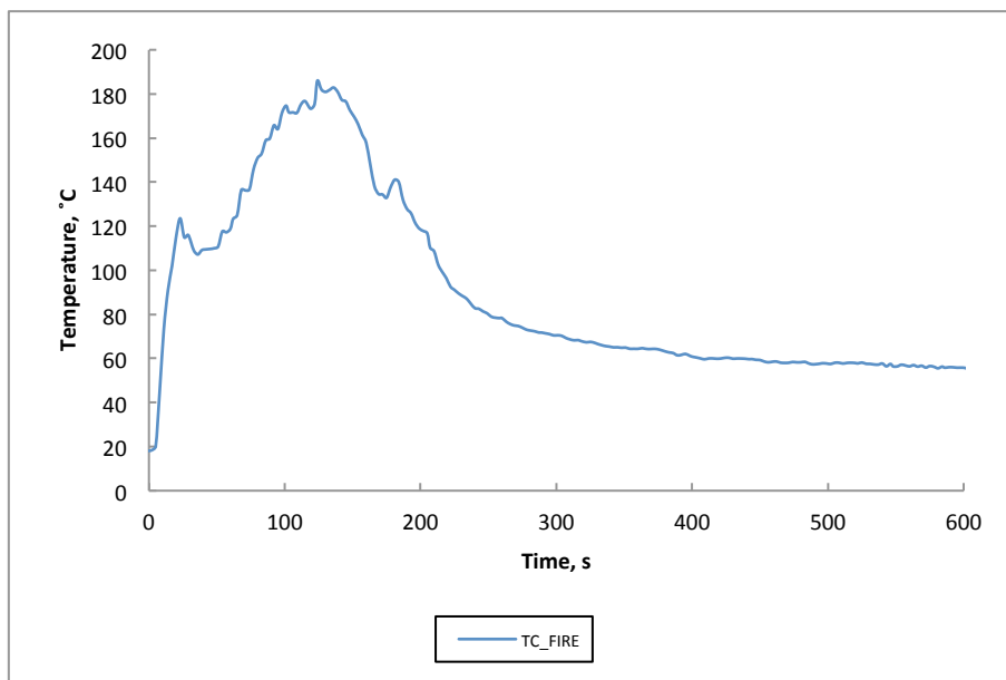
Figure 72 Temperature close to the pool fire, test 6.
