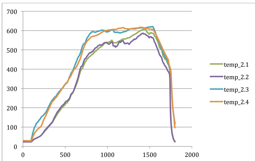
Figure 48 Measurement of temperatures inside steel bar number 2 in test P1.
