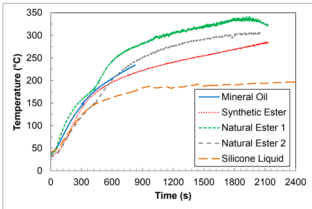
Figure 53 Liquid temperature at 1 cm below the surface in the tests with a round cup
