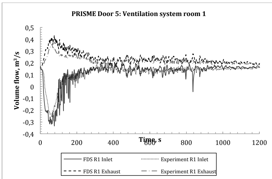
Figure 26 The predicted flow rates at inlet and exhaust in the fire compartment compared to the experimental data from test Door 5 (D5).
