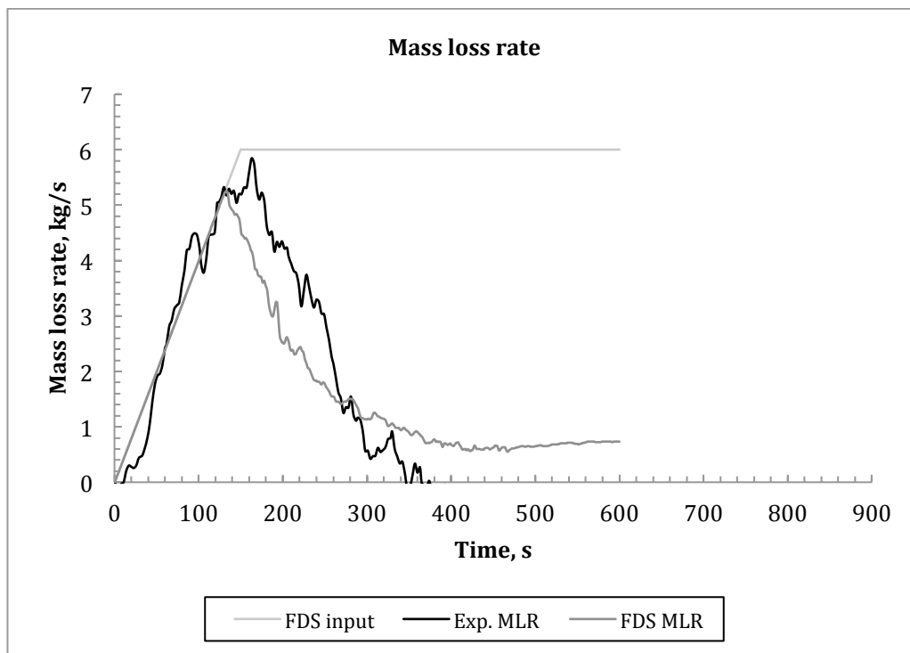
Figure 75 Simulation of mass loss rate for Ringhals test nr 6 and comparison with test
