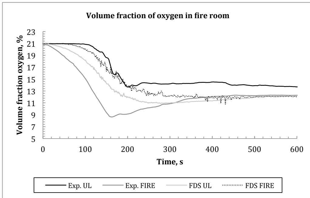
Figure 76 Simulation of oxygen volume fraction rate for Ringhals test nr 6 and comparison with test data
