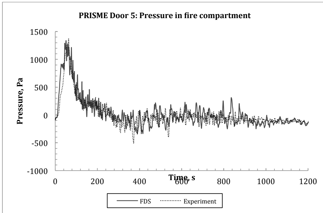
Figure 25 The predicted pressure inside the fire compartment compared to the experimental data from test Door 5 (D5).
