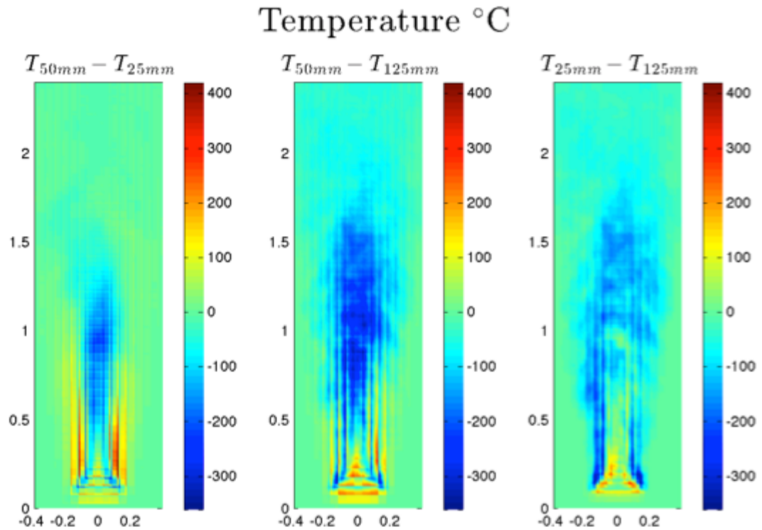
Figure 41. Differences between temperature slices at three different resolutions
