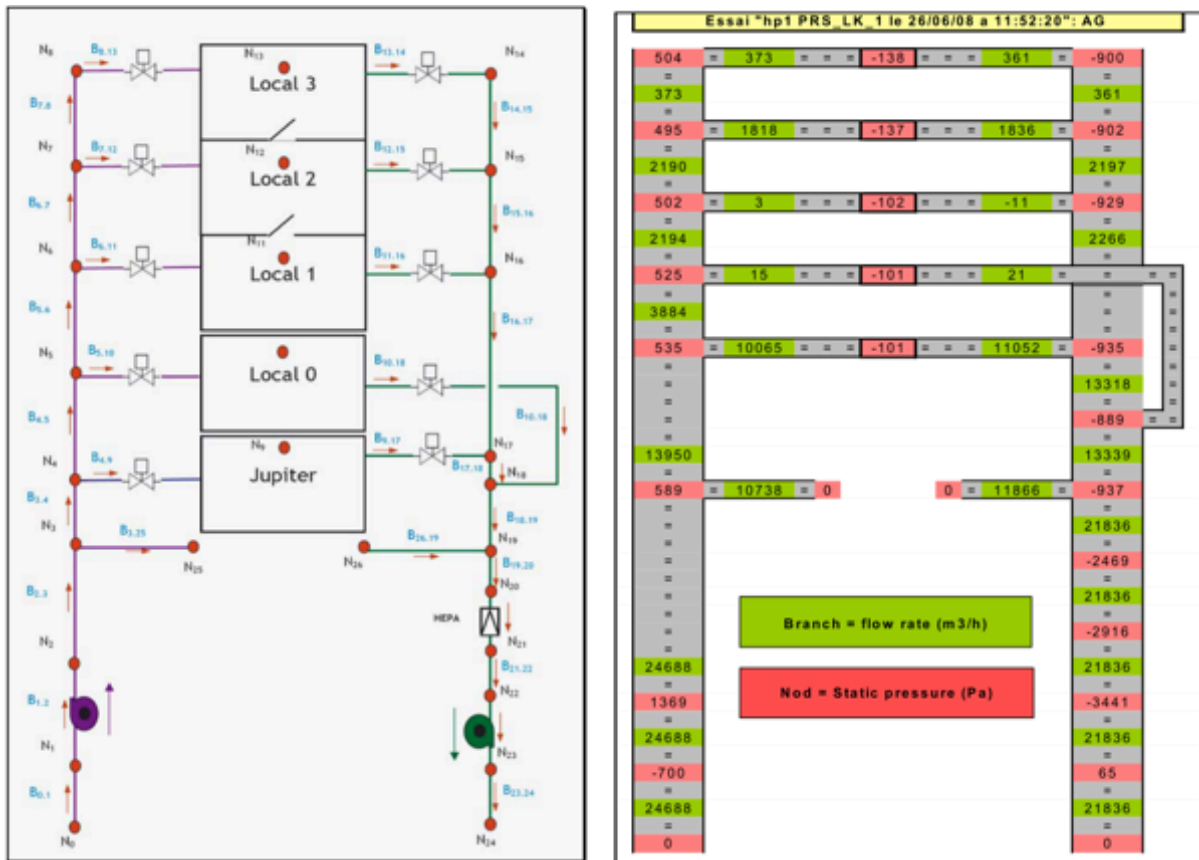
Figure 14 Initial ventilation data before ignition for PRISME Leak 1. Figure courtesy of IRSN.
