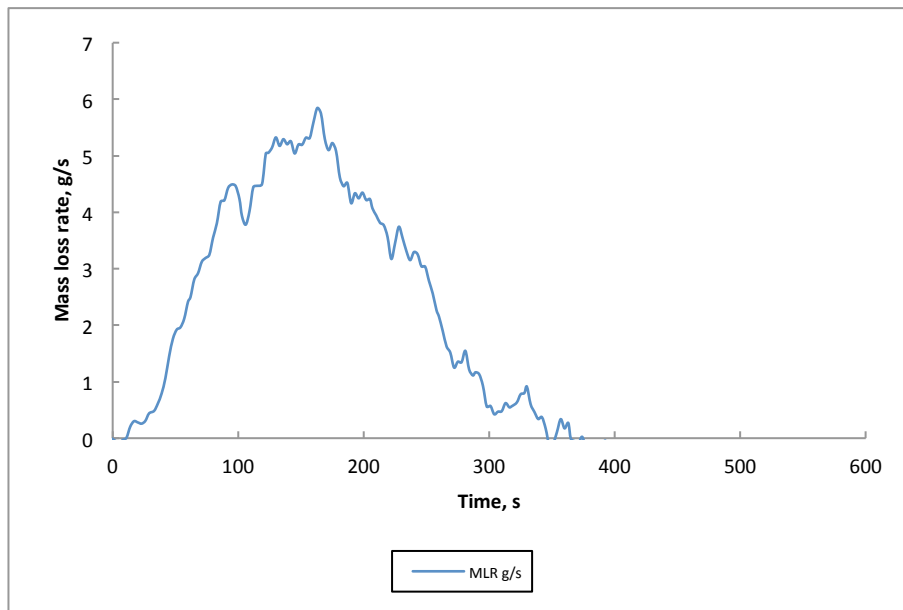
Figure 74 Mass loss rate of the pool fire containing heptane, test 6.
