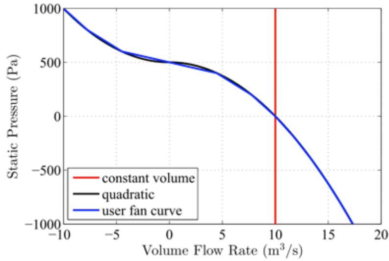
Figure 15 Example of a resulting fan curve when using the quadratic fan model built into FDS (39).
