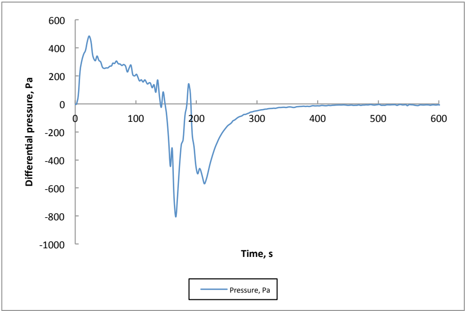
Figure 70 Pressure in the fire room, test 6.
