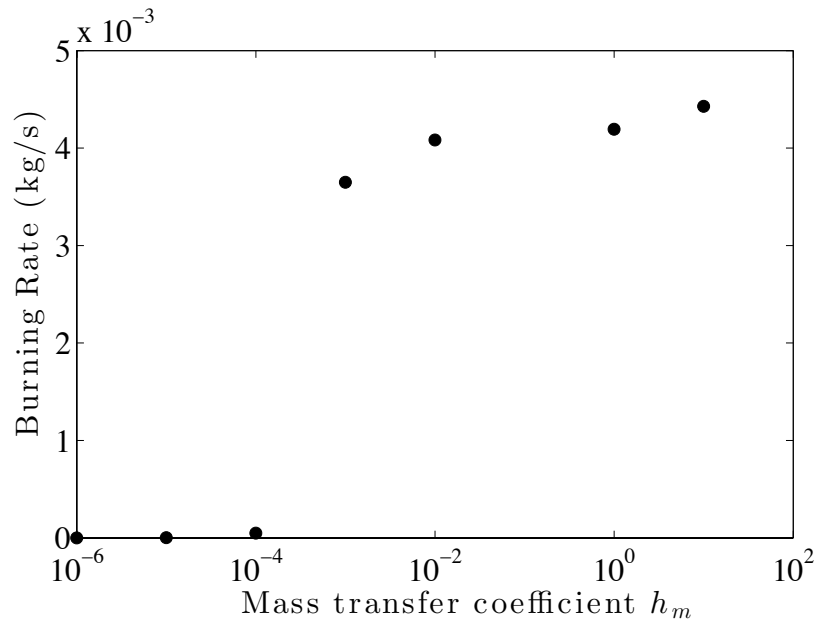
Figure 38 Sensitivity of pool fire burning rate predictions to the mass transfer coefficient.
