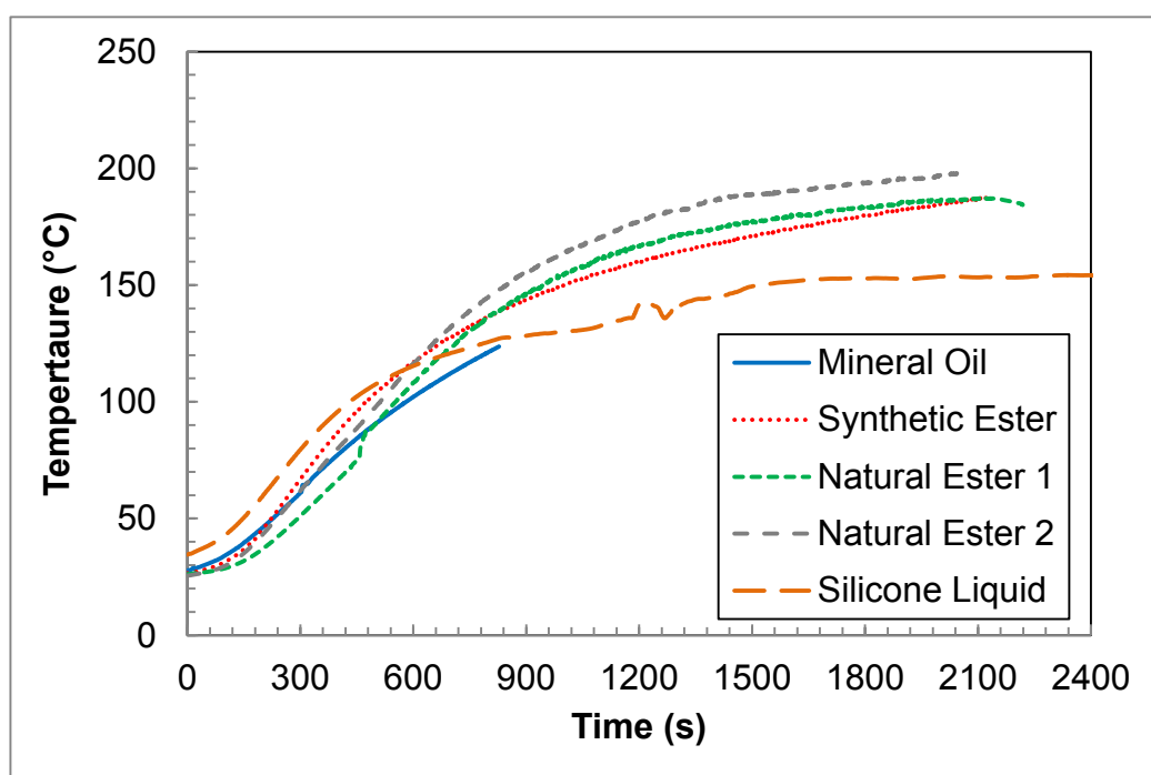
Figure 54 Liquid temperature at 3 cm below the surface in the tests with a round cup
