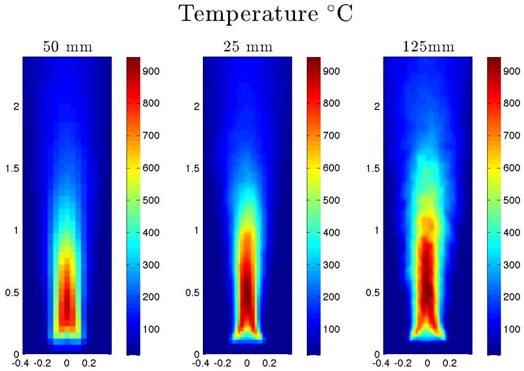
Figure 40. Temperature slices for three different grid resolutions.
