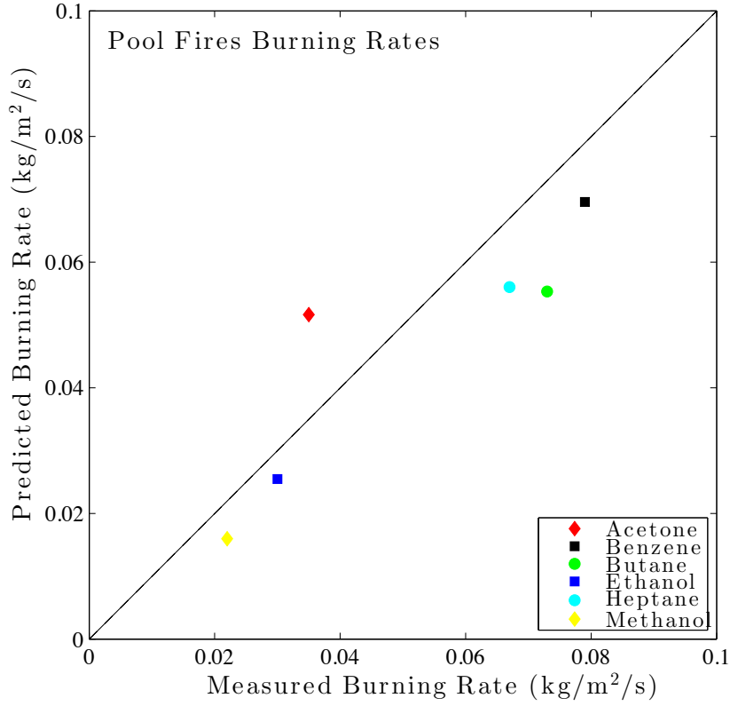
Figure 55. Maximum burning rates of large liquid pool fires
