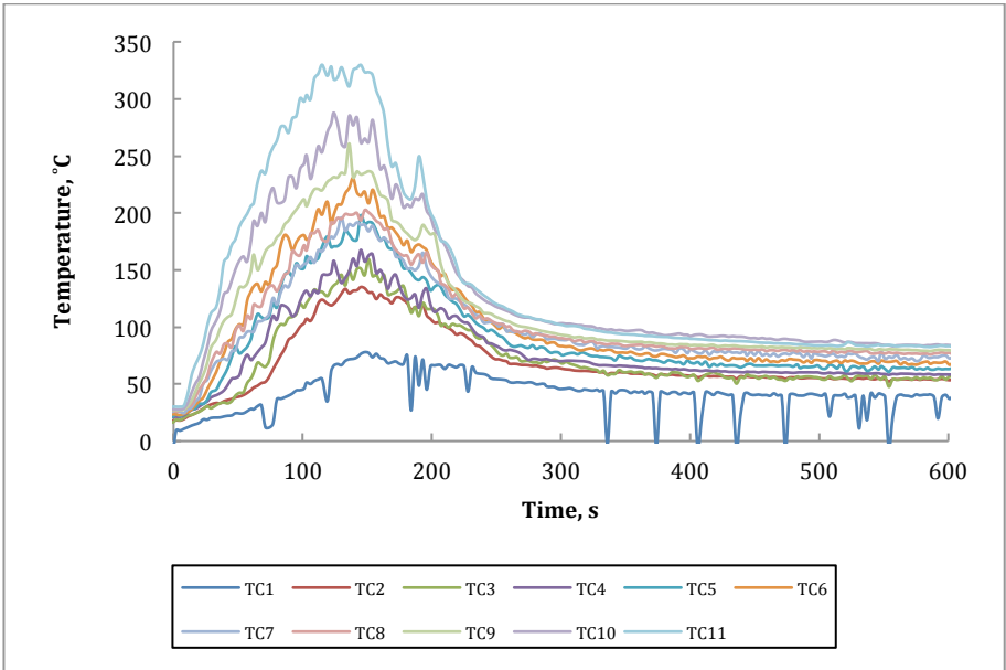
Figure 71 Temperatures in the thermocouple tree placed inside the fire room, test 6.
