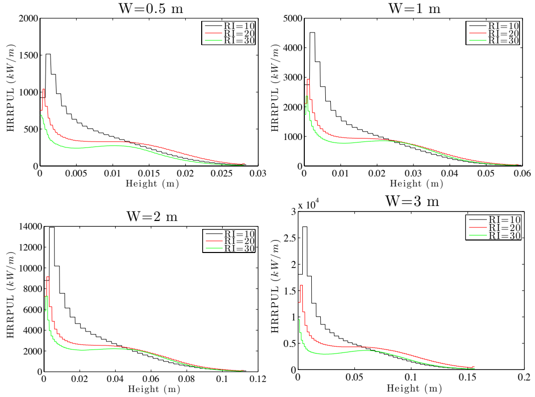
Figure 44. Heat Release Rate per Unit Length as function of height from floor. Fuel surface is at z=0.05 .
