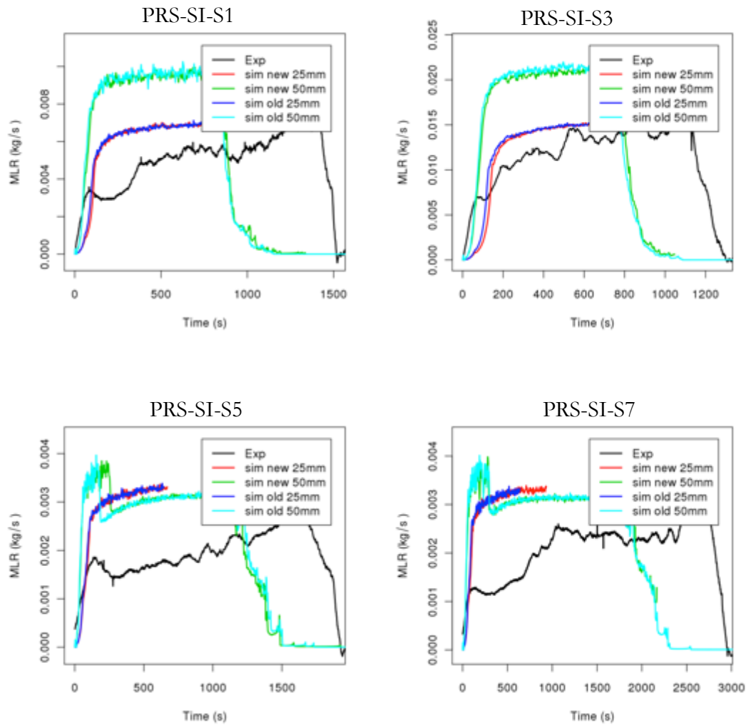
Figure 37 Comparison of pool evaporation models and different grid resolutions.
