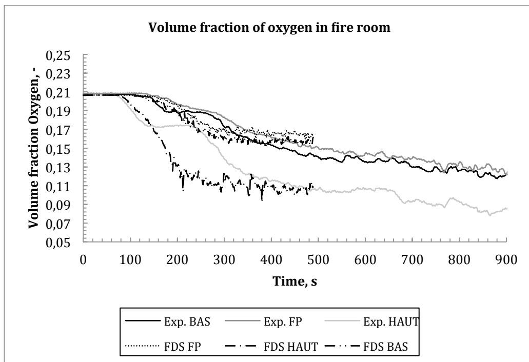
Figure 63 Prediction and test results of the oxygen volume fraction during LEAK1 test
