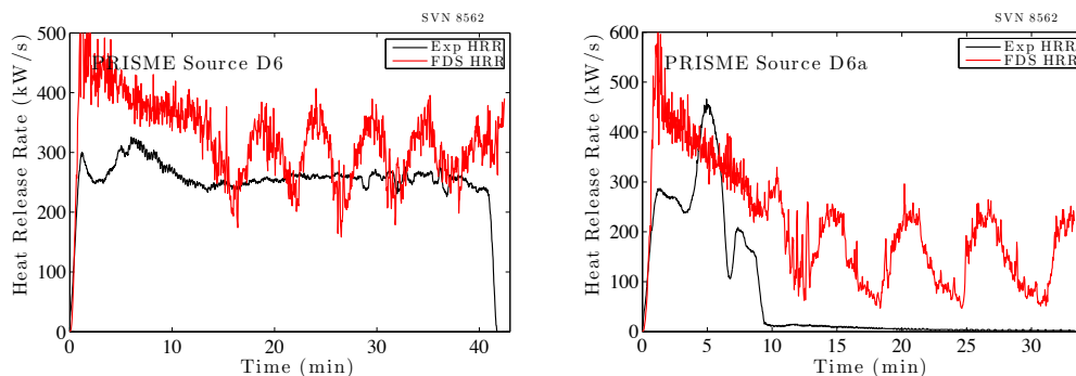
Figure 61. Predicted Heat Release Rates for PRISME source D6 and D6a tests. Both tests show oscillations in the predicted HRR and extinction due to lack of oxygen in D6a is not predicted.
