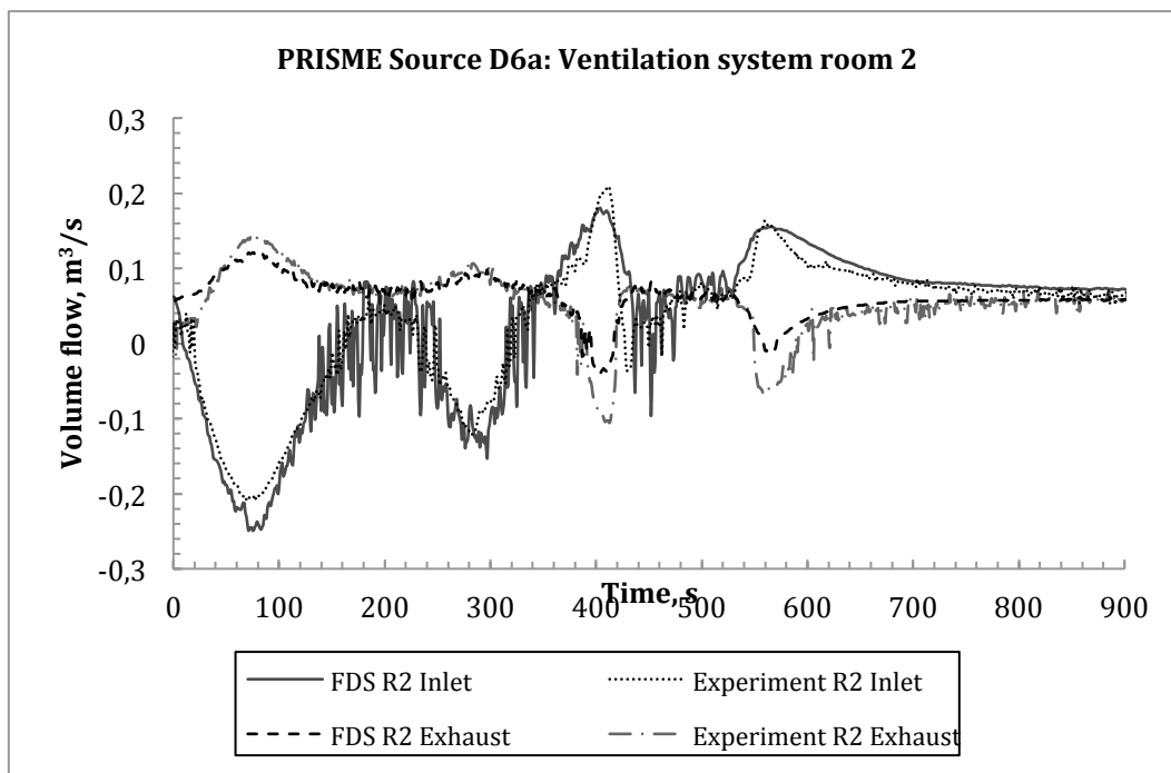
Figure 21 The predicted flow rates at inlet and exhaust in the fire compartment compared to the experimental data from test Source D6a (SI_D6a).
