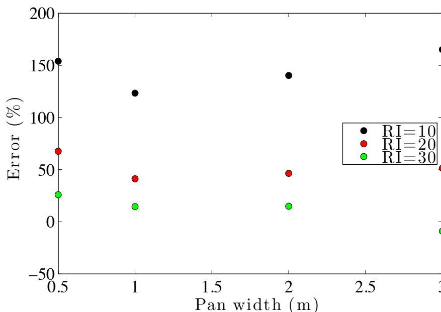
Figure 58. Error in predicted heat flux to burner surface as function of pan width and Resolution Index (RI)
