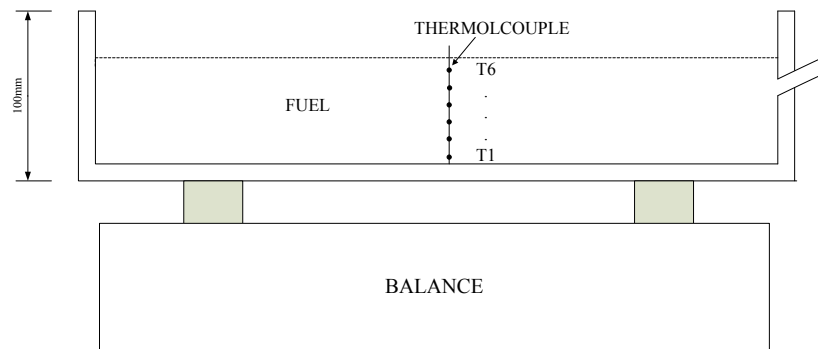
Figure 49 Schematic diagram of pool fire experimental set-up of fuel source
