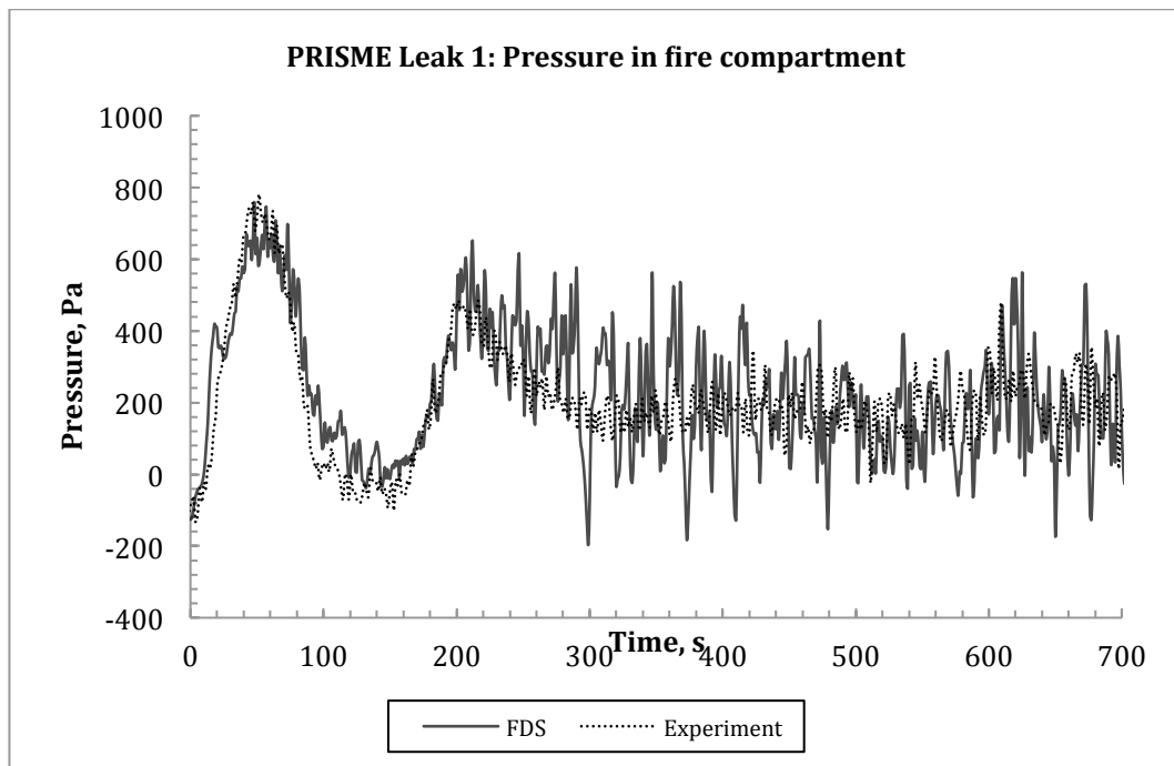
Figure 32 The predicted pressure inside the fire compartment compared to the experimental data from test Leak 1 (LK1).
