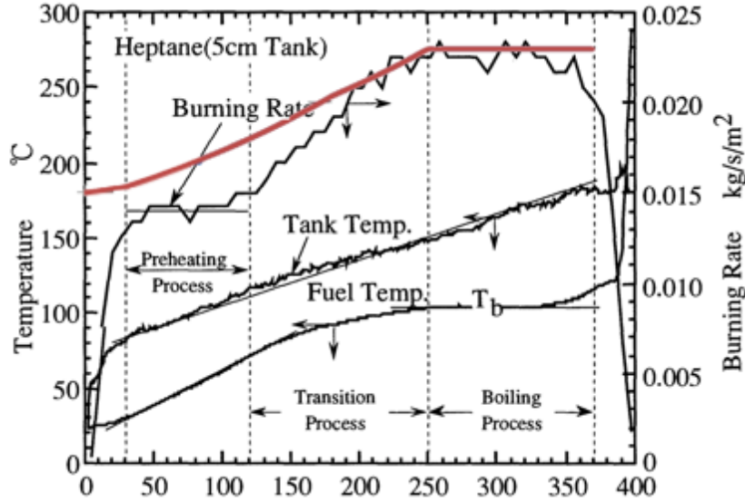
Figure 45 Comparison between experiments performed by Hayasaka (49) and the simple model to describe the initial phase of the pool fire. (reproduced from 49)
