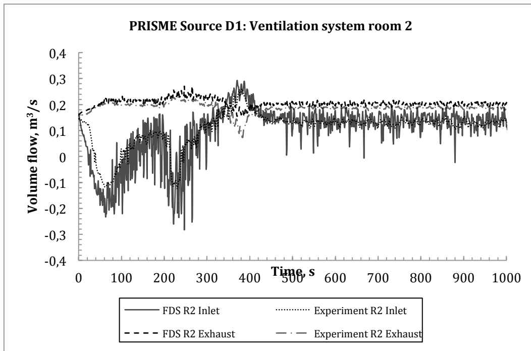
Figure 17 The predicted flow rates at inlet and exhaust in the fire compartment compared to the experimental data from test Source D1 (SI_D1).
