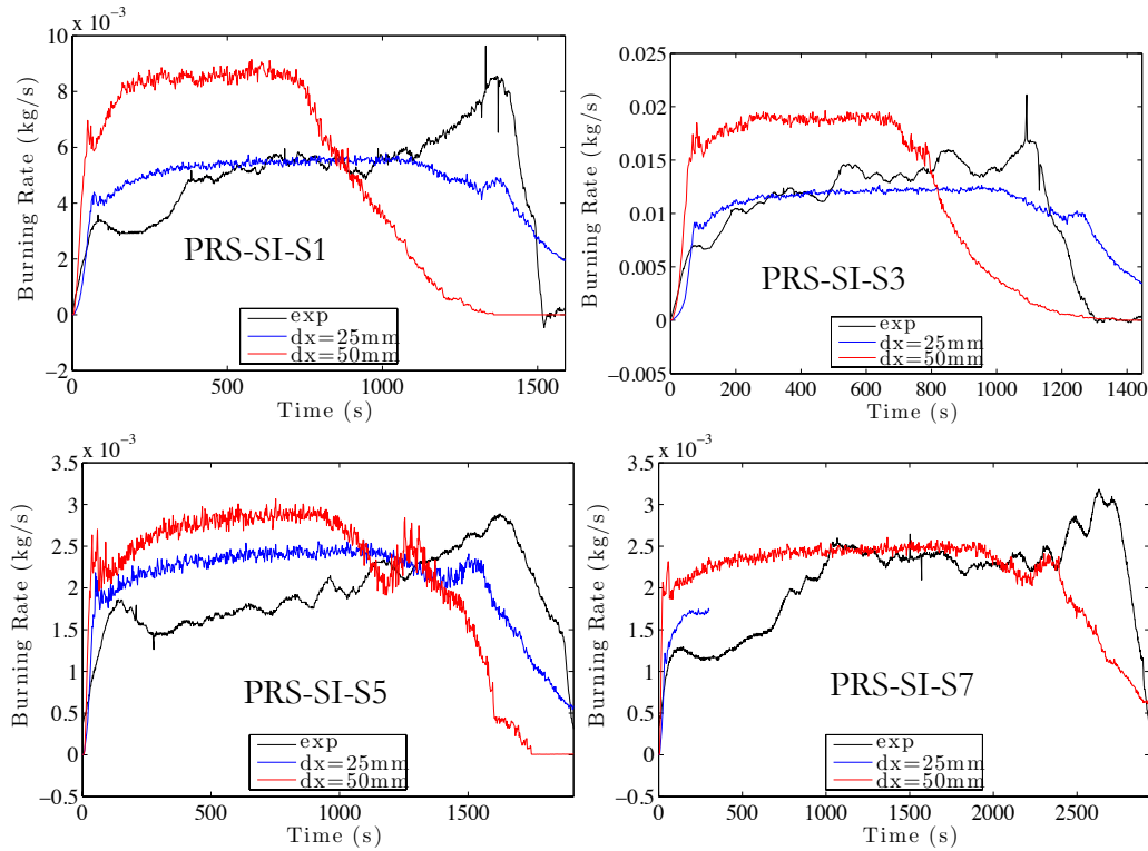
Figure 59. Comparison of predicted burning rates and experimental results
