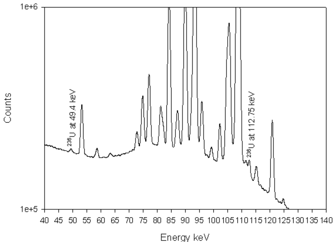
Figure 17. The 40 to 140 keV region of the Scenario 7 spectrum with the two ^{236}\text{U} peaks indicated.
