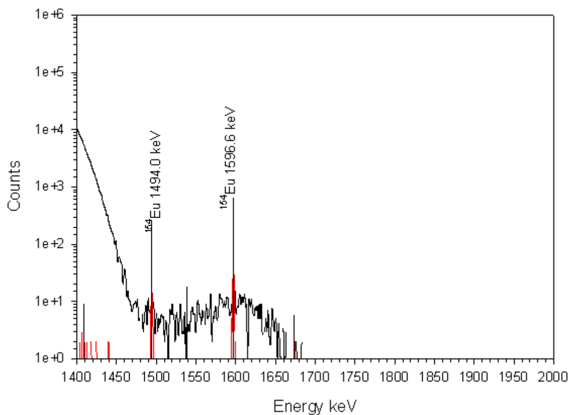
Figure A4. Assignment of constituent peaks for the spectrum of Scenario 4 (black) and the corresponding HPGGe spectrum (red).
