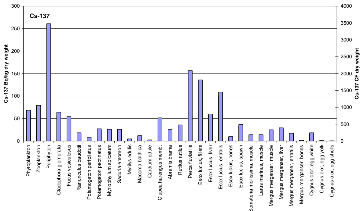
Figure 4. Mean values for ^{137}\text{Cs} ( \text{Bq kg}^{-1} dry weight) and mean concentration factors (on dry weight basis) in certain indicator samples in the sea area off Olkiluoto in 2001.
