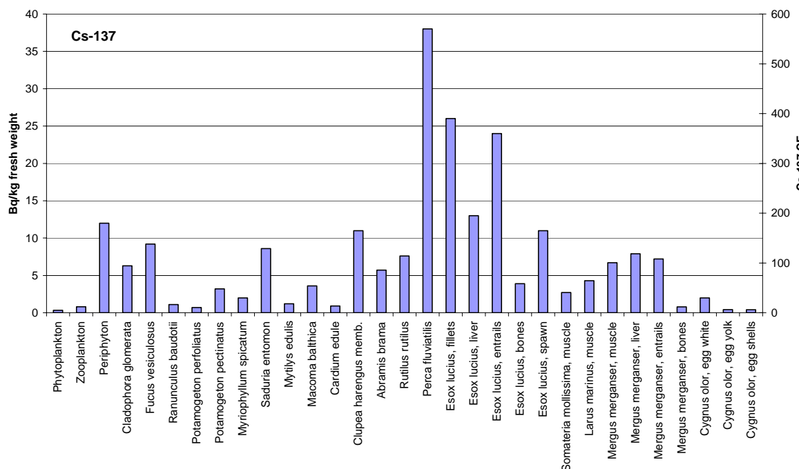
Figure 5. Mean values for ^{137}\text{Cs} ( \text{Bq kg}^{-1} fresh weight) and mean concentration factors (on fresh weight basis) in certain indicator samples in the sea area off Olkiluoto in 2001.
