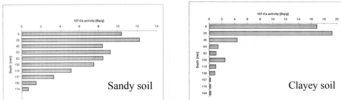
Figure 1. Vertical radiocaesium profiles in two soils in the Bryansk region. Samples taken 10 years after the Chernobyl accident contaminated the area.
