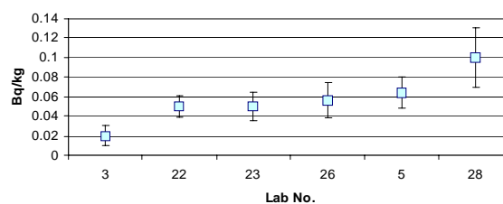
Am-241 in Mineral Matrix III
