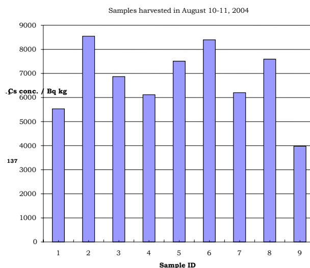
Figure 2. ^{137}\text{Cs} contents in perch (Samples 1-8) and pike (Sample 9) from lake Hedsjön, Gävle, Sweden.
