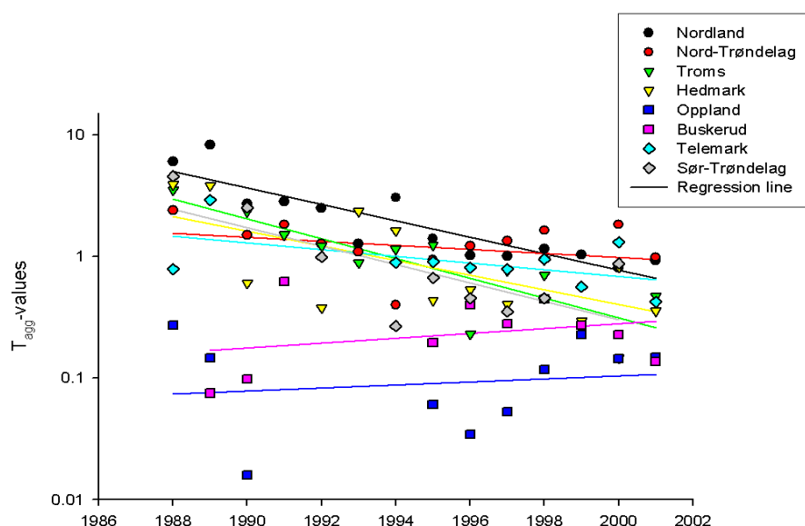
Figure 7. The relation between ground deposition of ^{137}\text{Cs} ( \text{Bq m}^{-2} ) and the activity concentration of ^{137}\text{Cs} in lynx muscle ( \text{Bq kg}^{-1} ) in 1988-2001. Calculated aggregated transfer coefficient ( T_{\text{agg}} , \text{m}^2 \text{kg}^{-1} ) for different counties in Norway.
