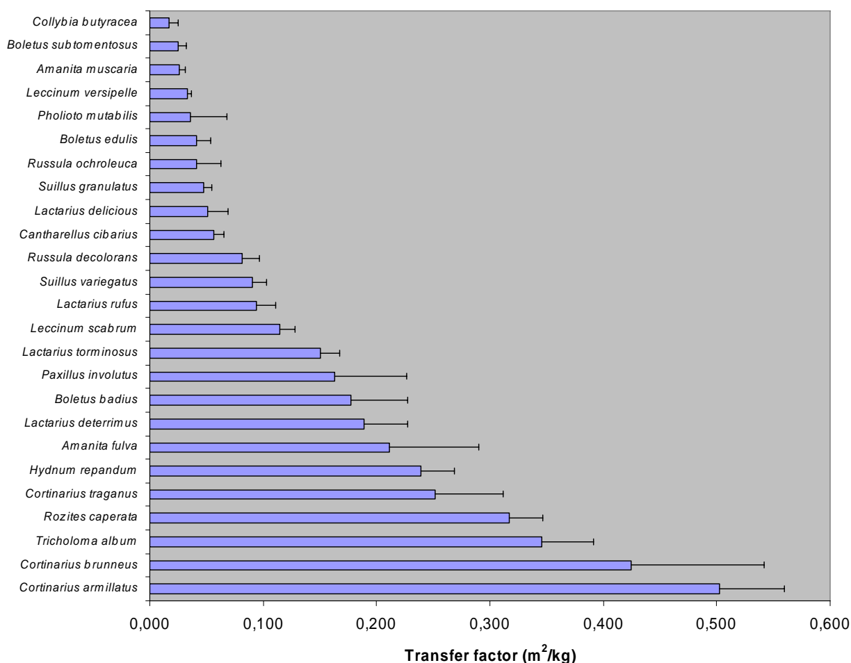
Figure 2. Mean transfer factor of 137 Cs (m 2 kg -1 fresh wt.) with standard deviation in different fungi species (n=1283) in Norway in 1988-2002.
