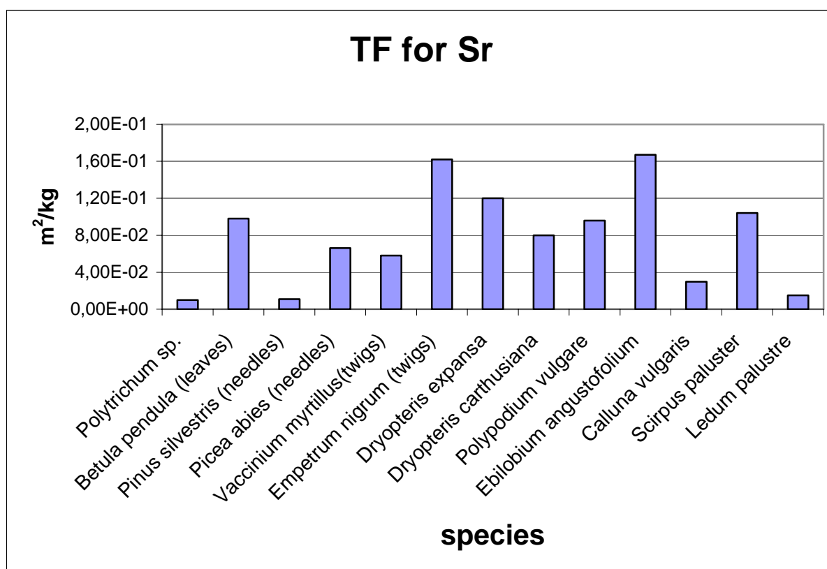
Figure 7. Aggregated transfer factors of Sr-90 for certain terrestrial plants except mushrooms.
