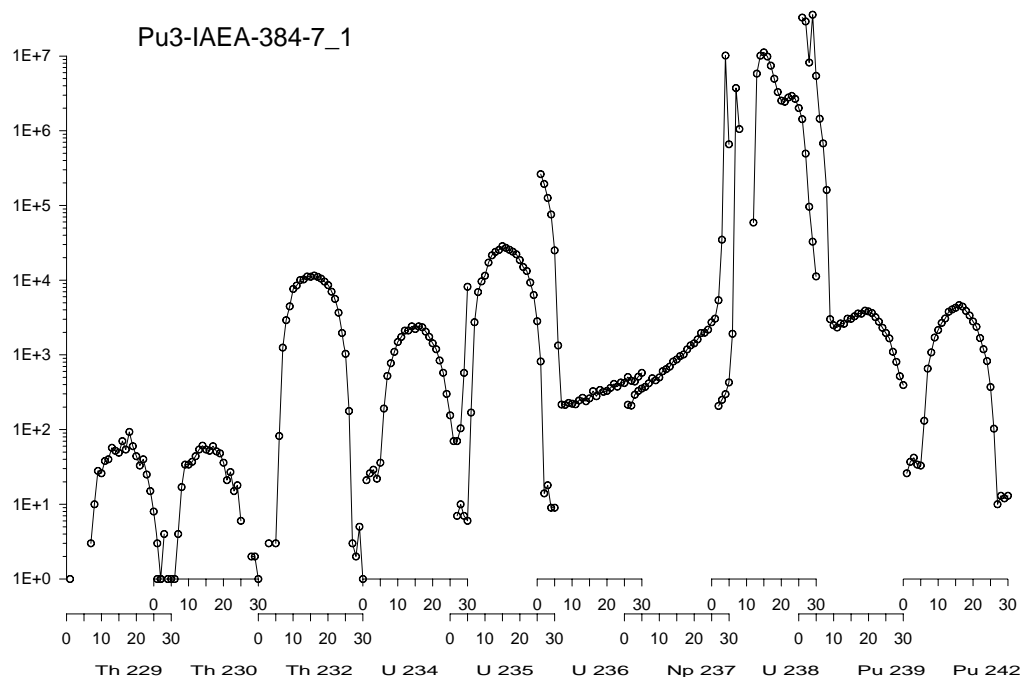
Figure 1. Mass-spectrum of a radiochemically purified sample of the reference material IAEA-384 (coral from Muroroo). The purified sample was analysed by alpha spectrometry, then stripped from the disc and measured by ICP-MS. Pu-242 was used as a yield determinant.
