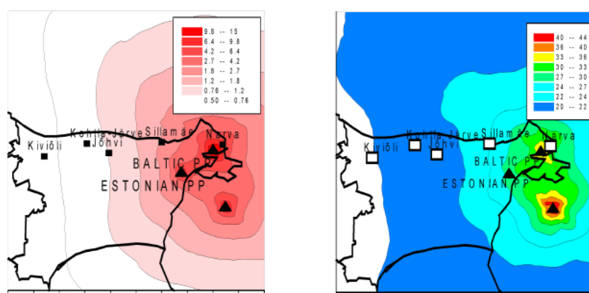
Figure 3. ^{210}\text{Pb} deposition flux ( \text{Bq m}^{-2} \text{a}^{-1} ) and annual doses ( \text{Sv/a} ). The CAP88PC atmospheric transfer modelling software was utilised including local ash data (1995), radioactive ash contents and long-term local meteorology.
