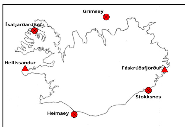
Figure 2. Seaweed sampling sites at the Icelandic coast (Circles: Fucus vesiculosus ; triangles: Ascophyllum nodosum ).
