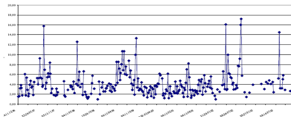
Figure 6. Radiocaesium concentrations ( \text{Bq/m}^3 ) in air in Narva-Jõesuu, 1997-2003.
