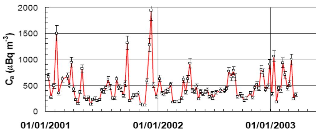
Figure 4. Weekly 210 Pb activity concentration (σBq m -3 ) in near-surface air, Narva-Jõesuu, 2001-2003.
