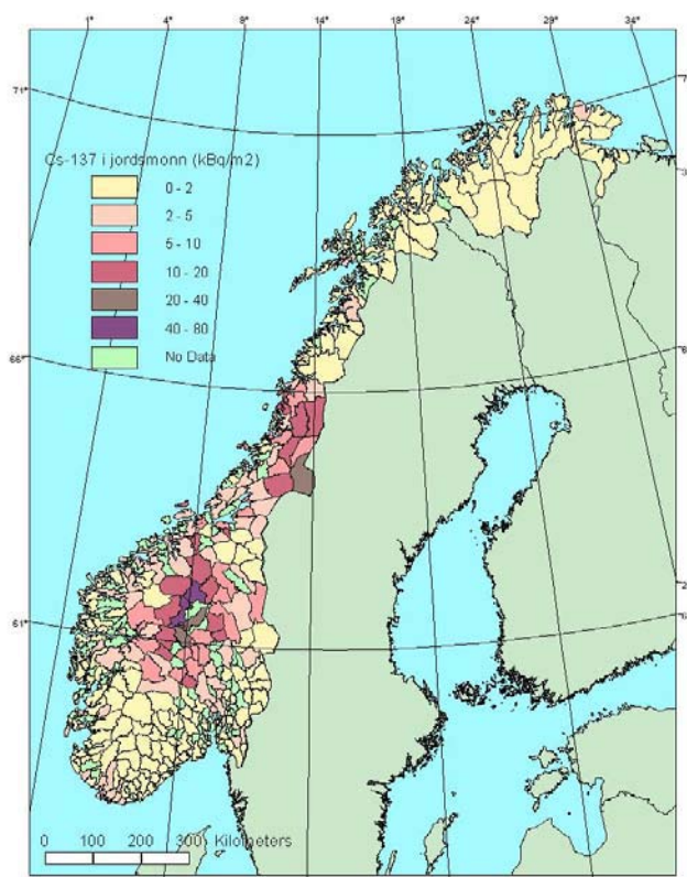
Figure 1. Ground deposition of ^{137}\text{Cs} in different municipalities in Norway, 1. July 1995.
