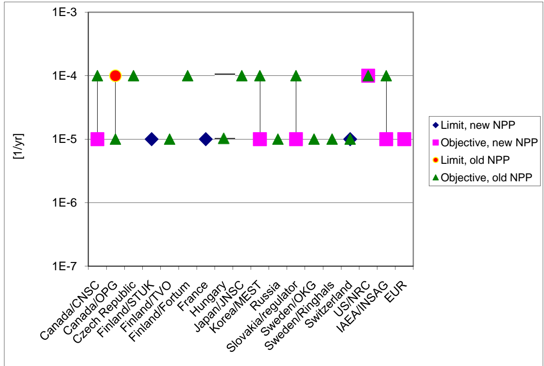
Figure 4 Numerical criteria defined for core damage.
