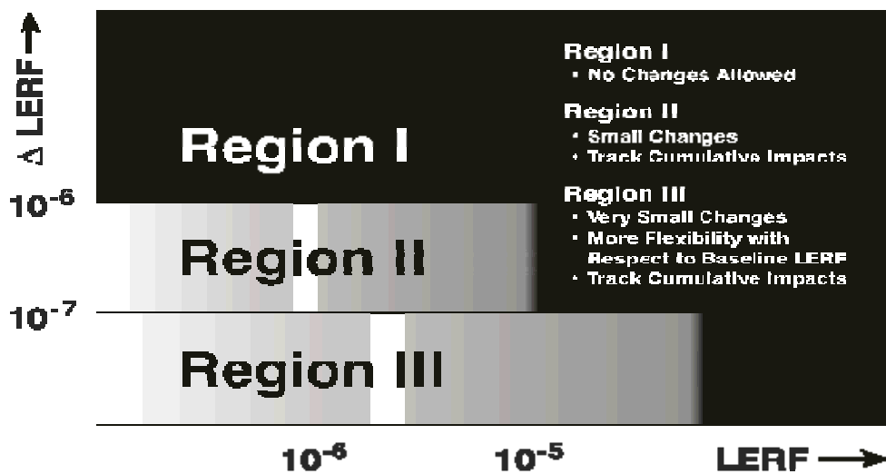
Figure 5 RG 1.174 Acceptance Guidelines for Large Early Release Frequency (LERF).
