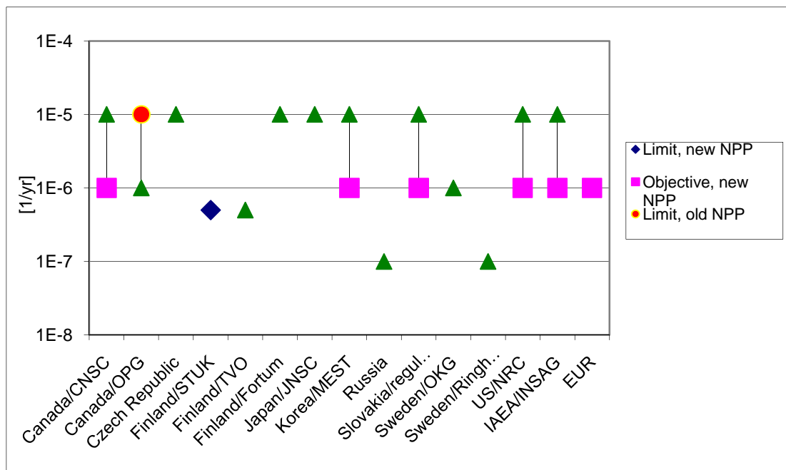
Figure 3 Numerical criteria defined for large release. Definition and timing of “large release” varies.
